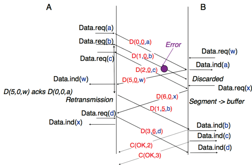
Figure 4.23: Piggybacking
