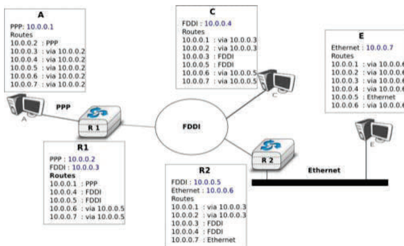
Figure 5.19: Scalability issues when using isolated IP addresses
