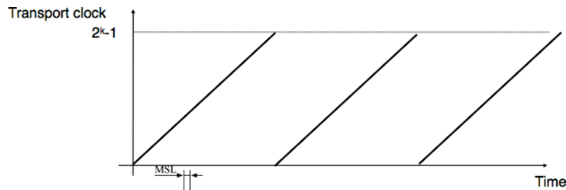
Figure 4.27: Transport clock
