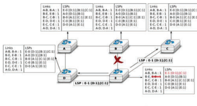
Figure 5.16: The two-way connectivity check
