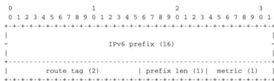
Figure 5.49: Format of the RIP IPv6 route entries
