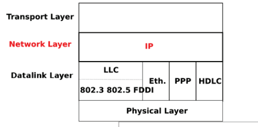
Figure 5.18: IP and the reference model
