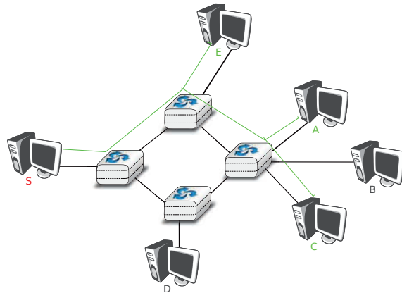
Figure 2.10: Multicast transmission
