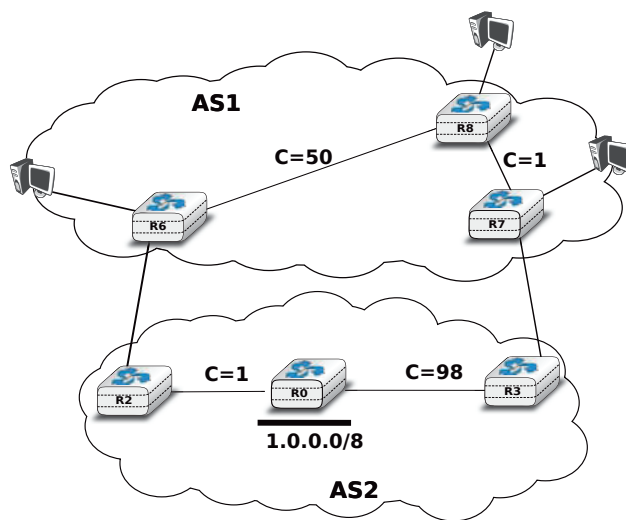
Figure 5.69: Hot and cold potato routing
